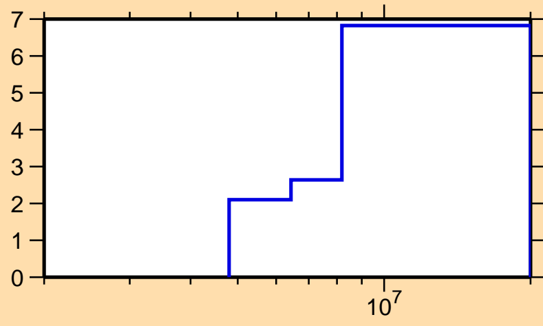
\Delta\sigma/\sigma vs. E for ^{114}\text{Cd}(n,\text{inel.})
