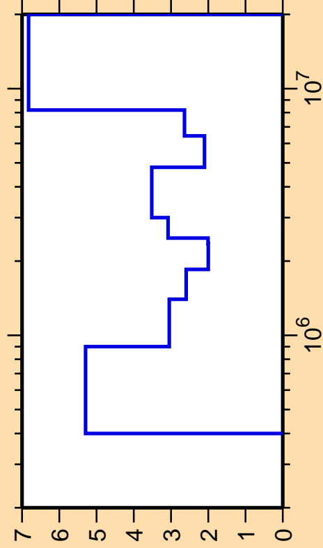
\Delta\sigma/\sigma vs. E for ^{114}\text{Cd}(n,\text{inel.})
