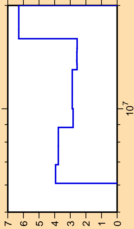
\Delta\sigma/\sigma vs. E for ^{115}\text{Cd}(n,2n)
