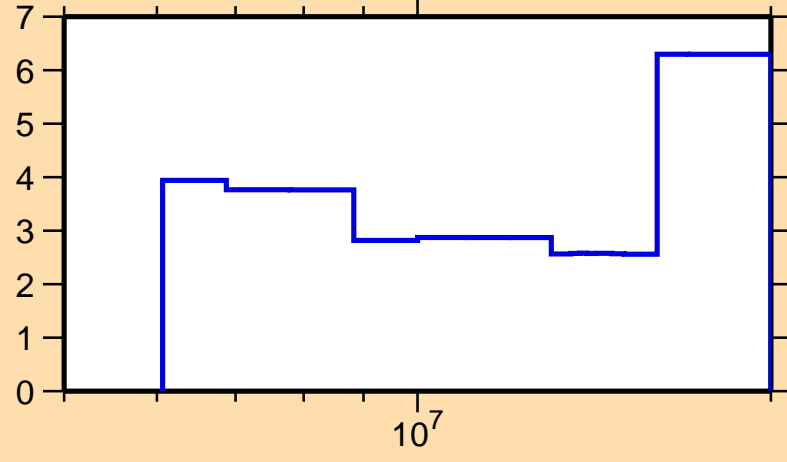
\Delta\sigma/\sigma vs. E for ^{115}\text{Cd}(n,2n)
