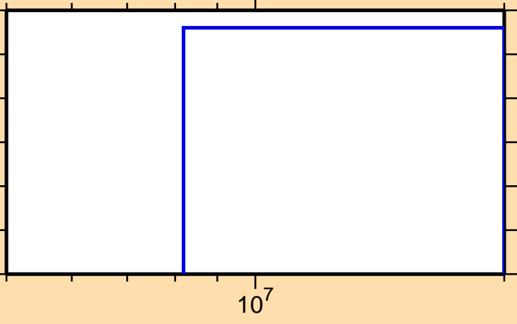
\sigma vs. E for ^{115}\text{Cd}(n,nt)
