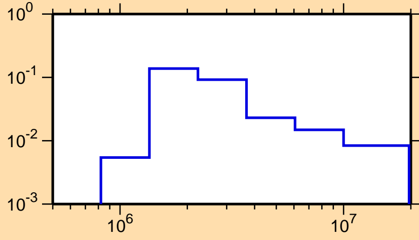
\sigma vs. E for ^{116}\text{Cd}(n,n_3)
