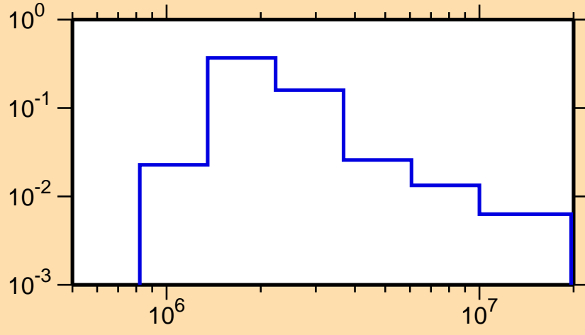
\sigma vs. E for ^{116}\text{Cd}(n,n_2)
