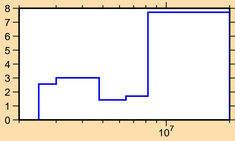
\Delta\sigma/\sigma vs. E for ^{116}\text{Cd}(n,\text{inel.})
