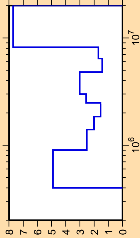
\Delta\sigma/\sigma vs. E for ^{116}\text{Cd}(n,\text{inel.})
