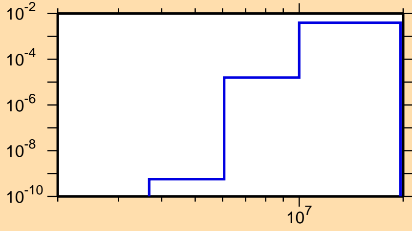
\sigma vs. E for ^{117}\text{Cd}(n,p)
