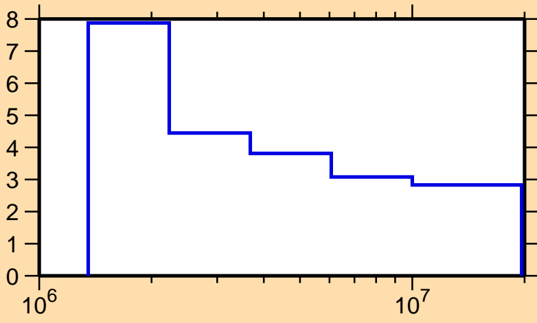
\Delta\sigma/\sigma vs. E for ^{117}\text{Cd}(n,n\text{onel.})
