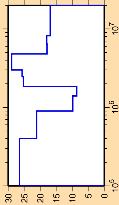
\Delta\sigma/\sigma vs. E for ^{117}\text{Cd}(n,n_4)
