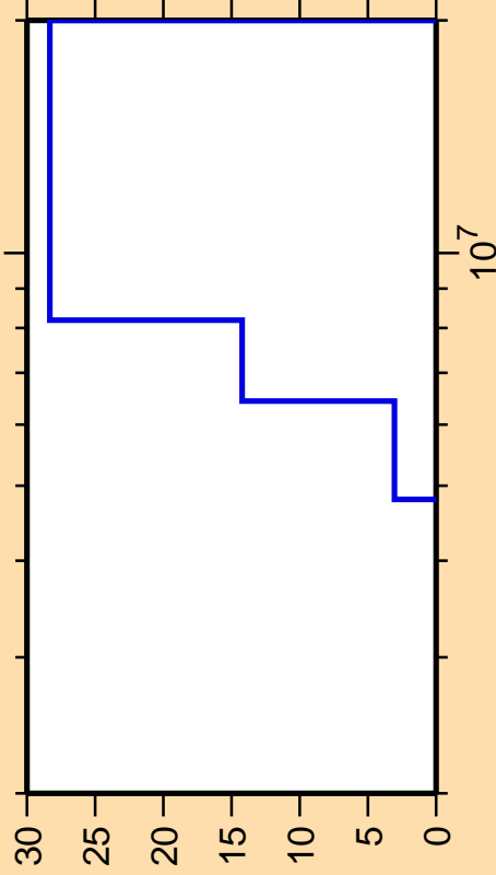
\Delta\sigma/\sigma vs. E for ^{117}\text{Cd}(n,n\text{cont.})
