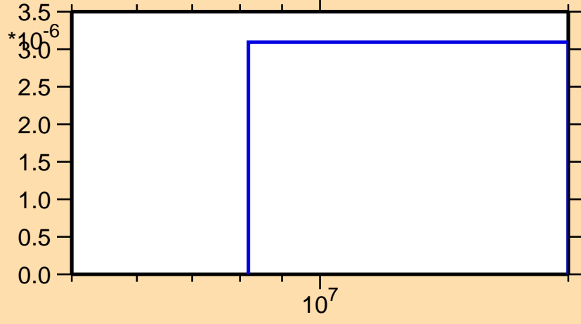
\sigma vs. E for ^{117}\text{Cd}(n,n\alpha)
