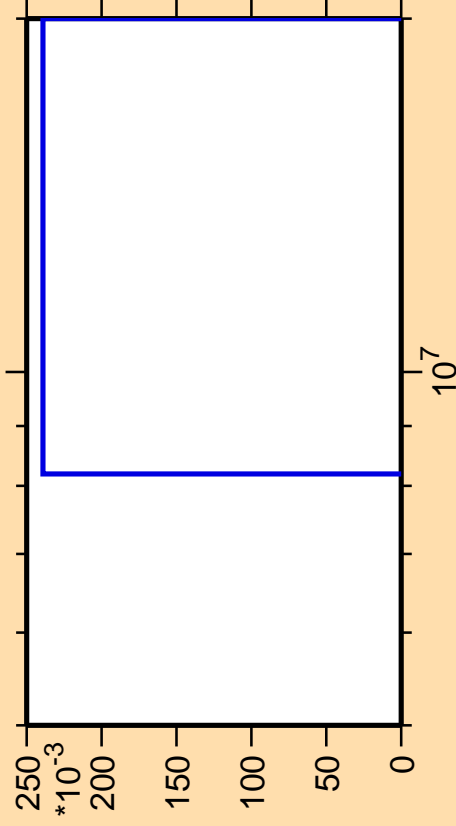
\Delta\sigma/\sigma vs. E for ^{117}\text{Cd}(n,nt)
