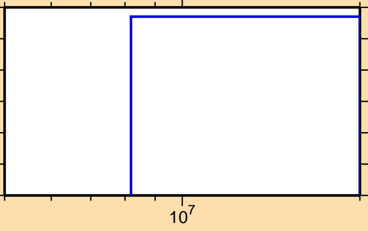
\sigma vs. E for ^{117}\text{Cd}(n,t)
