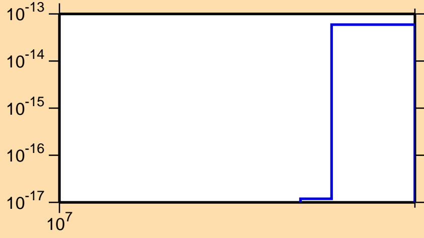
\sigma vs. E for ^{118}\text{Cd}(n,2n\alpha)
