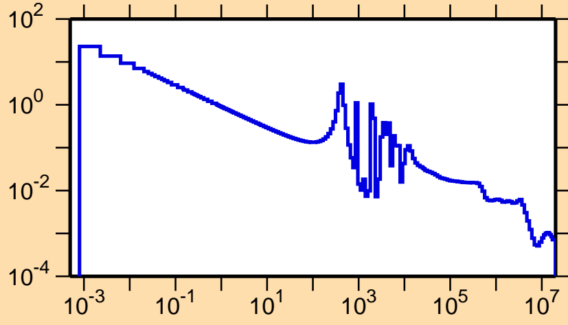
\sigma vs. E for ^{118}\text{Cd}(n,\gamma)
