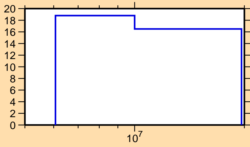
\Delta\sigma/\sigma vs. E for ^{118}\text{Cd}(n,n_1)
