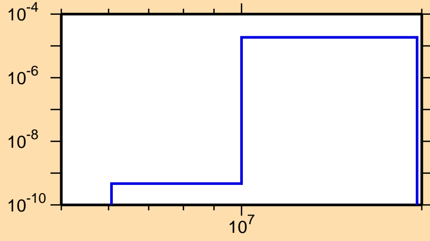
\sigma vs. E for ^{118}\text{Cd}(n,\alpha)
