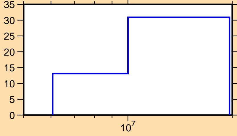
\Delta\sigma/\sigma vs. E for ^{118}\text{Cd}(n,ncont.)
