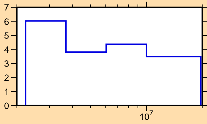
\Delta\sigma/\sigma vs. E for ^{118}\text{Cd}(n,\text{el.})
