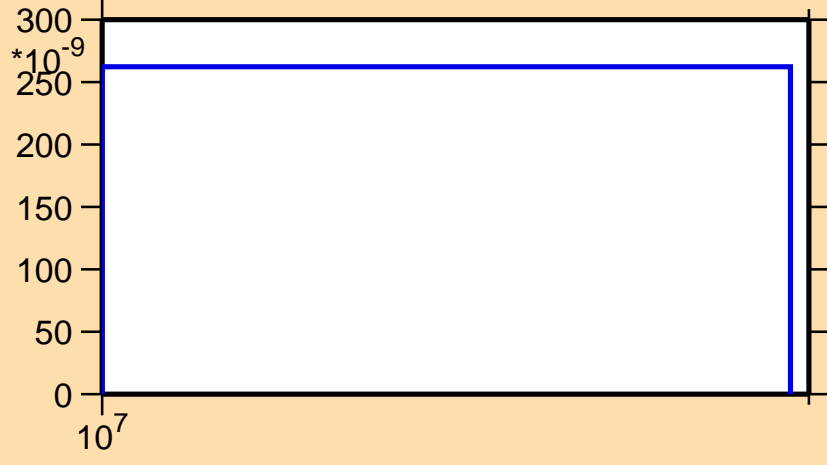
\sigma vs. E for ^{118}\text{Cd}(n,t)
