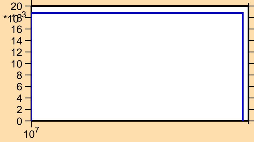
\sigma vs. E for ^{118}\text{Cd}(n,3n)
