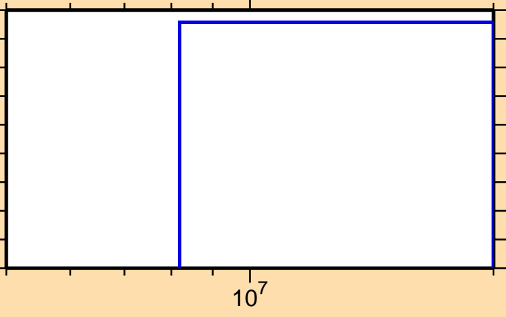
\sigma vs. E for ^{118}\text{Cd}(n,nt)
