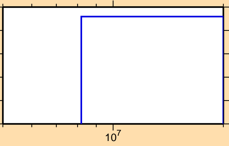
\sigma vs. E for ^{118}\text{Cd}(n,d)
