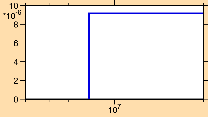
\sigma vs. E for ^{118}\text{Cd}(n,d)
