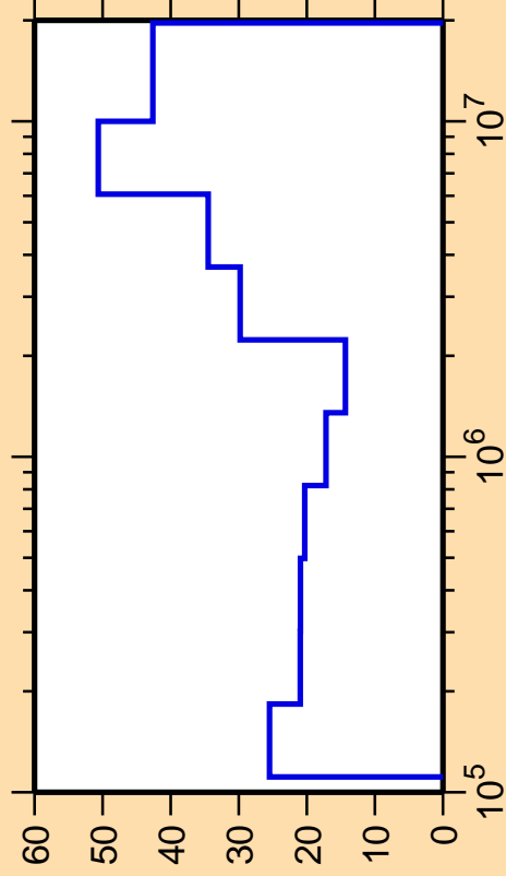
\Delta\sigma/\sigma vs. E for ^{119}\text{Cd}(n,n_2)
