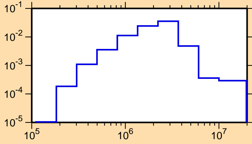
\sigma vs. E for ^{119}\text{Cd}(n,n_2)
