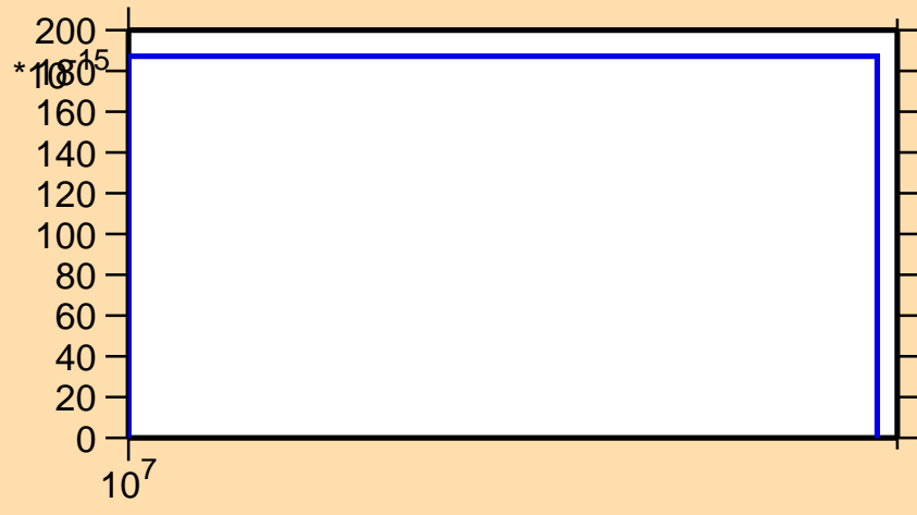
\sigma vs. E for ^{119}\text{Cd}(n,2np)
