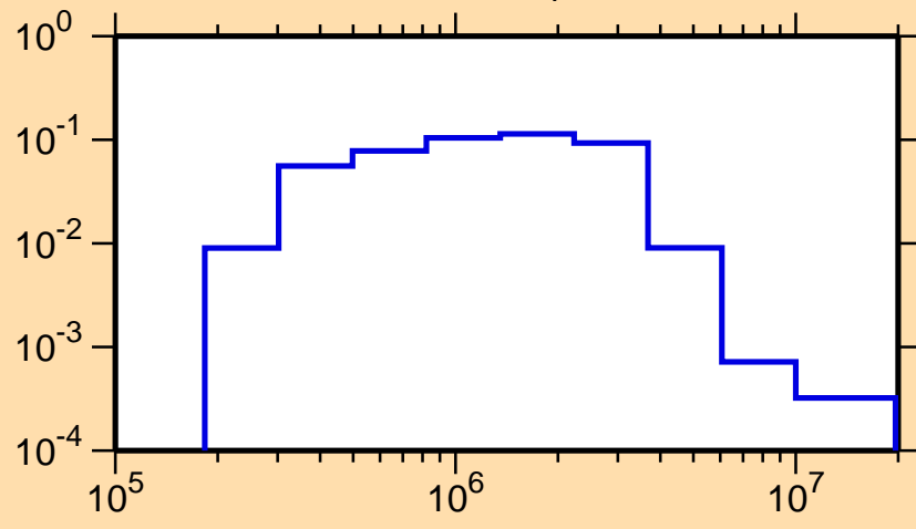
\sigma vs. E for ^{119}\text{Cd}(n,n_4)
