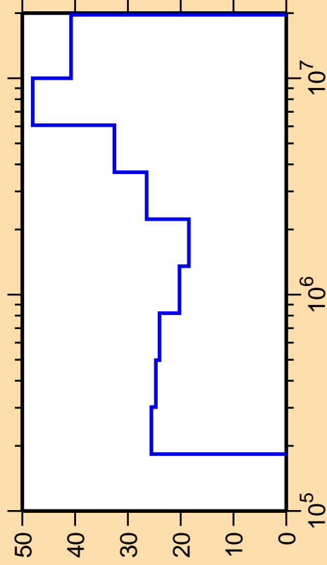
\Delta\sigma/\sigma vs. E for ^{119}\text{Cd}(n,n_4)
