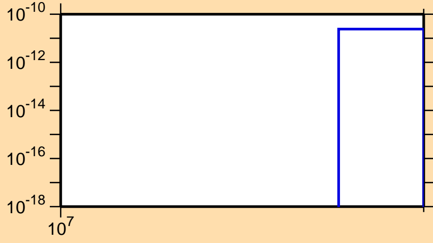
\sigma vs. E for ^{119}\text{Cd}(n,nt)
