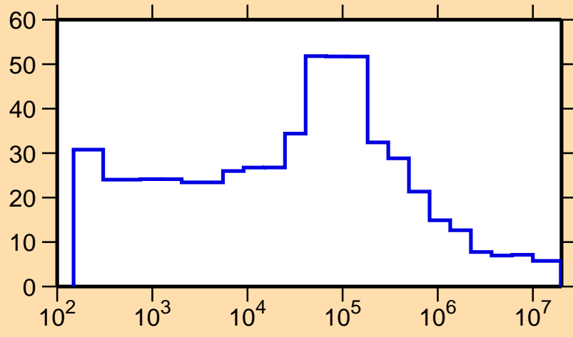
\Delta\sigma/\sigma vs. E for ^{119}\text{Cd}(n,\text{nonel.})
