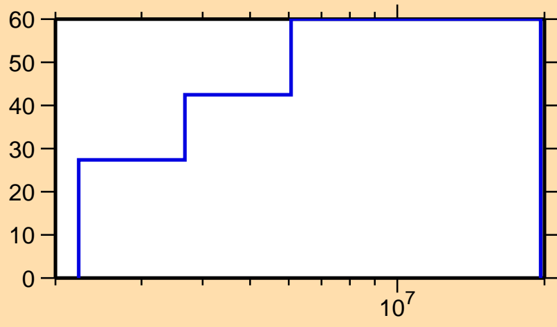
\Delta\sigma/\sigma vs. E for ^{119}\text{Cd}(n,n_1)
