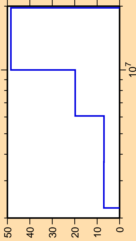
\Delta\sigma/\sigma vs. E for ^{119}\text{Cd}(n,n\text{cont.})
