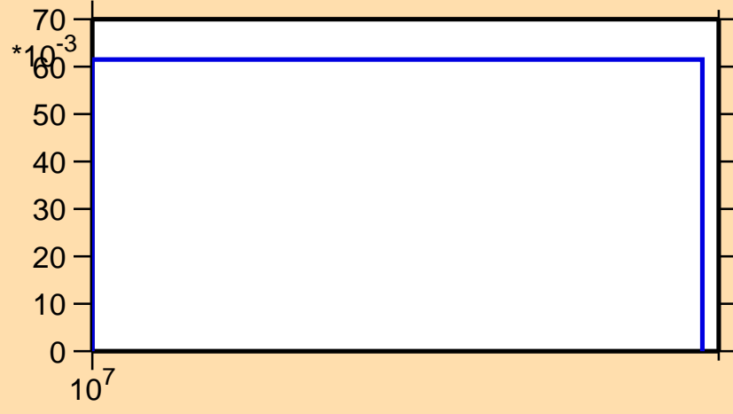
\sigma vs. E for ^{119}\text{Cd}(n,3n)
