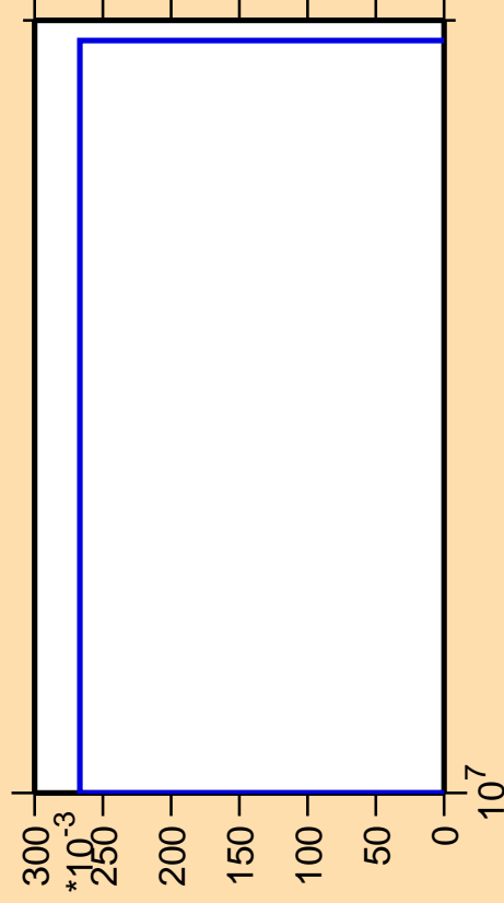
\Delta\sigma/\sigma vs. E for ^{119}\text{Cd}(n,2np)
