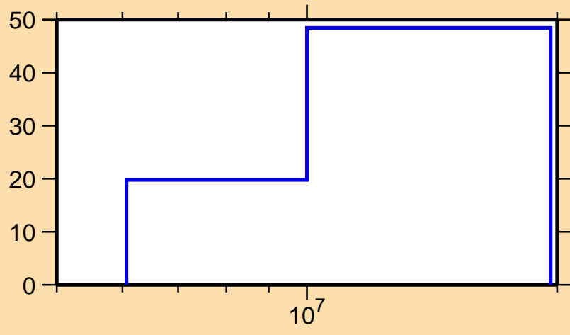
\Delta\sigma/\sigma vs. E for ^{119}\text{Cd}(n,ncont.)
