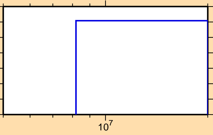
\sigma vs. E for ^{119}\text{Cd}(n,np)
