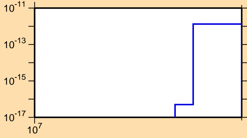
\sigma vs. E for ^{120}\text{Cd}(n,nt)
