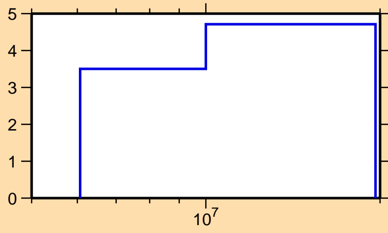
\Delta\sigma/\sigma vs. E for ^{120}\text{Cd}(n,\text{tot.})
