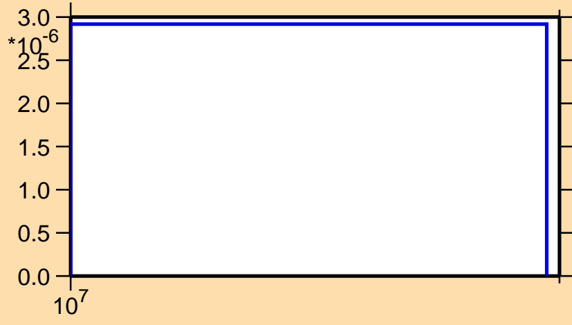
\sigma vs. E for ^{120}\text{Cd}(n,d)
