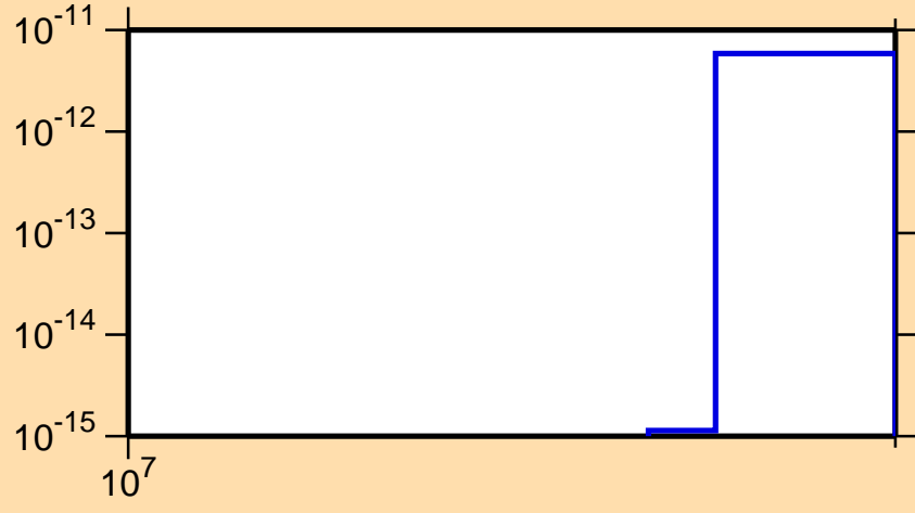
\sigma vs. E for ^{121}\text{Cd}(n,2n\alpha)
