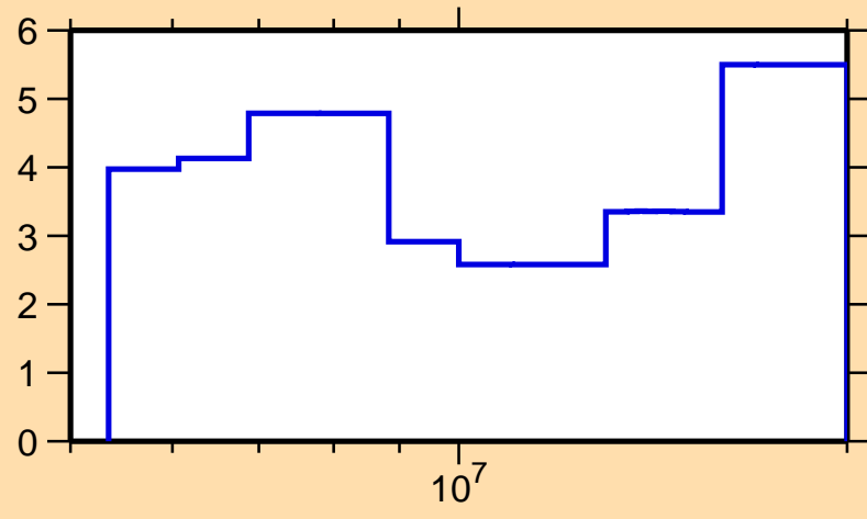
\Delta\sigma/\sigma vs. E for ^{121}\text{Cd}(n,\text{tot.})
