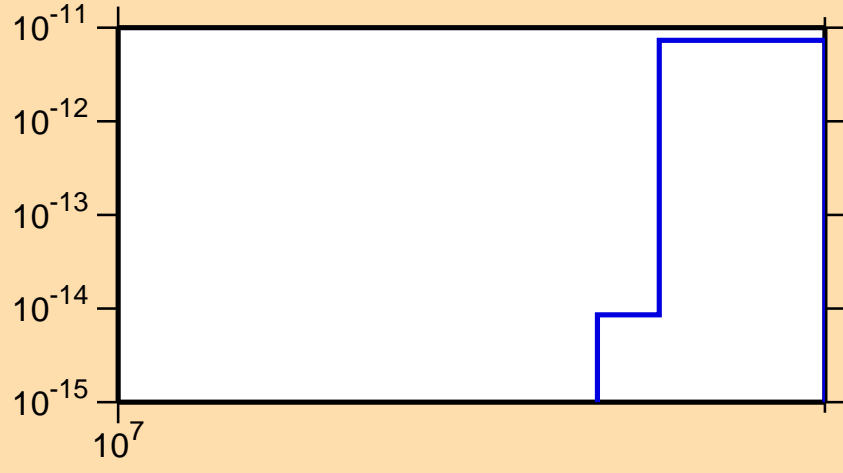
\sigma vs. E for ^{121}\text{Cd}(n,nt)
