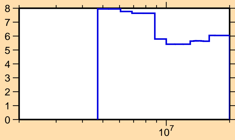
\Delta\sigma/\sigma vs. E for ^{121}\text{Cd}(n,\text{nonel.})
