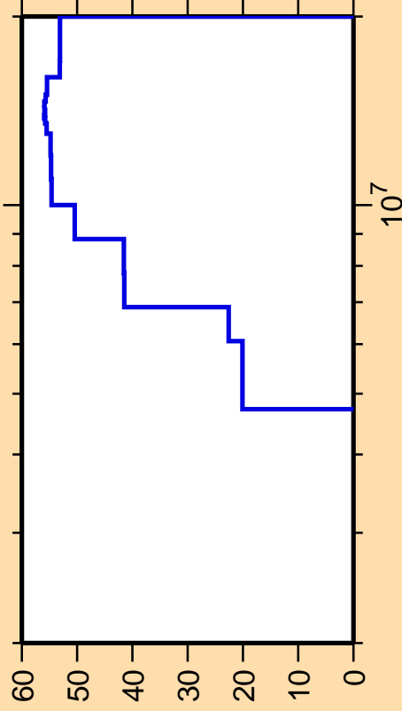
\Delta\sigma/\sigma vs. E for ^{121}\text{Cd}(n,n_{\text{cont}}) .
