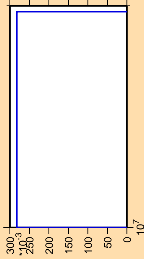
\Delta\sigma/\sigma vs. E for ^{121}\text{Cd}(n,nt)
