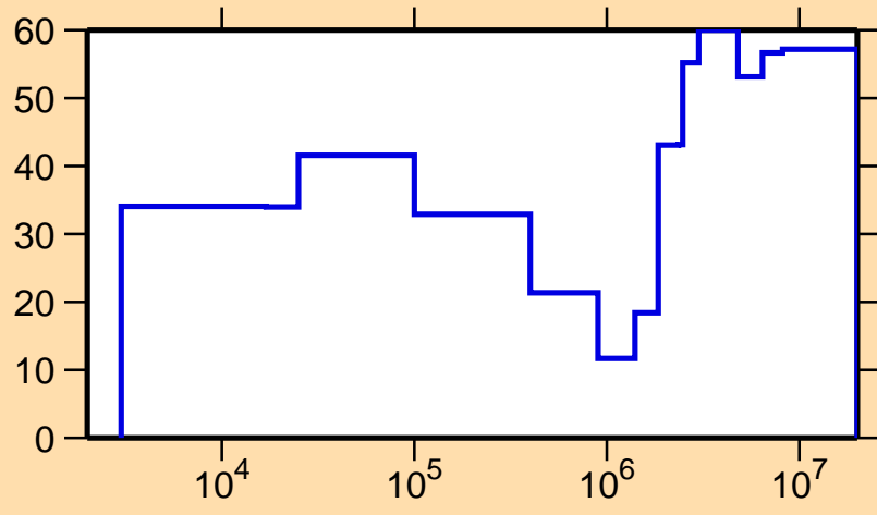
\Delta\sigma/\sigma vs. E for ^{121}\text{Cd}(n,n_1)
