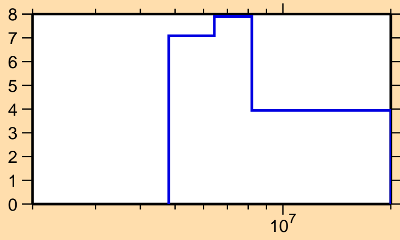
\Delta\sigma/\sigma vs. E for ^{121}\text{Cd}(n,\text{el.})
