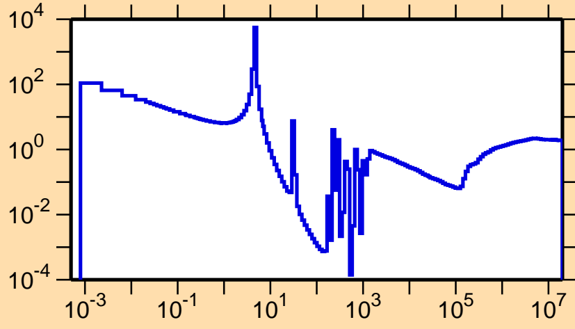
\sigma vs. E for ^{121}\text{Cd}(n,\text{nonel.})
