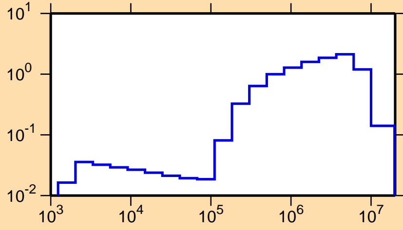
\sigma vs. E for ^{121}\text{Cd}(n,\text{inel.})
