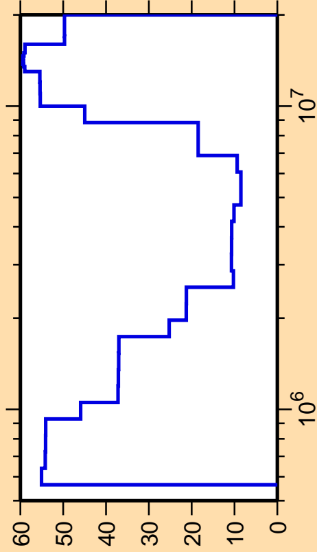
\Delta\sigma/\sigma vs. E for ^{122}\text{Cd}(n,\text{inel.})
