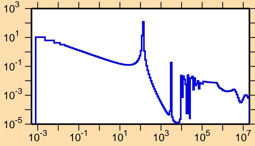
\sigma vs. E for ^{122}\text{Cd}(n,\gamma)
