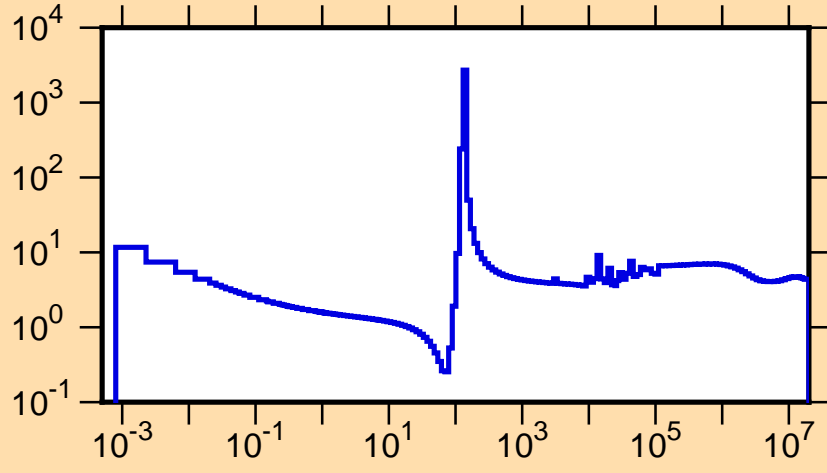
\sigma vs. E for ^{122}\text{Cd}(n,\text{tot.})
