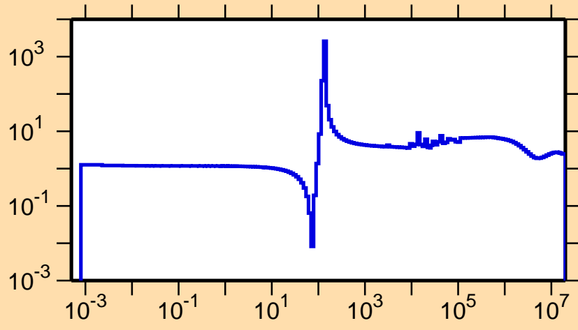
\sigma vs. E for ^{122}\text{Cd}(n,\text{el.})
