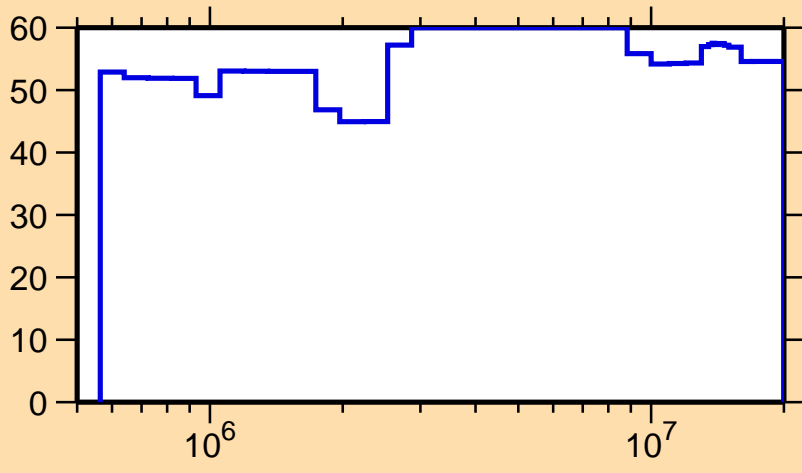
\Delta\sigma/\sigma vs. E for ^{122}\text{Cd}(n,n_1)
