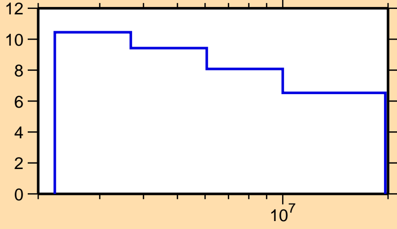
\Delta\sigma/\sigma vs. E for ^{122}\text{Cd}(n,n\text{onel.})
