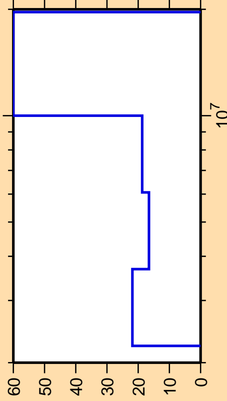
\Delta\sigma/\sigma vs. E for ^{122}\text{Cd}(n,n_{\text{cont}}) .
