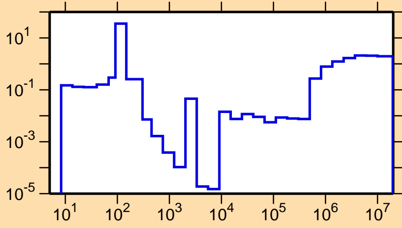
\sigma vs. E for ^{122}\text{Cd}(n,\text{nonel.})
