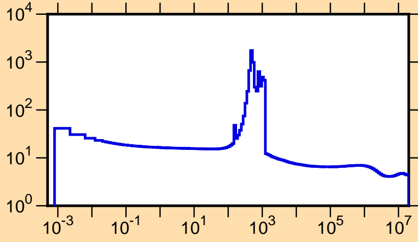
\sigma vs. E for ^{123}\text{Cd}(n,\text{tot.})
