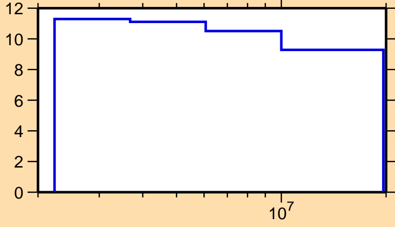
\Delta\sigma/\sigma vs. E for ^{123}\text{Cd}(n,n\text{onel.})
