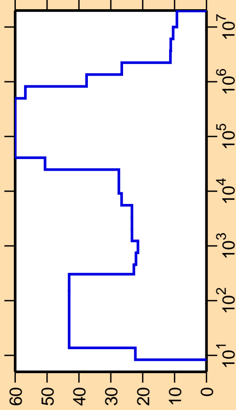
\Delta\sigma/\sigma vs. E for ^{123}\text{Cd}(n,\text{nonel.})
