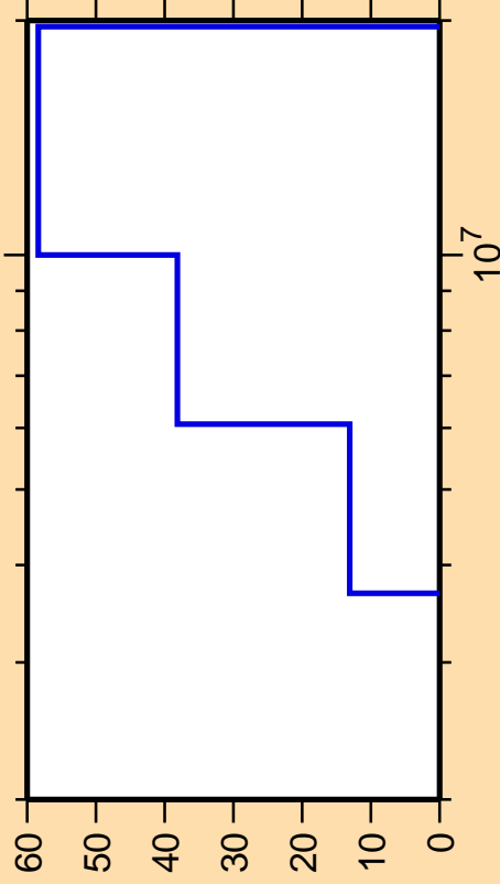
\Delta\sigma/\sigma vs. E for ^{123}\text{Cd}(n,n\text{cont.})
