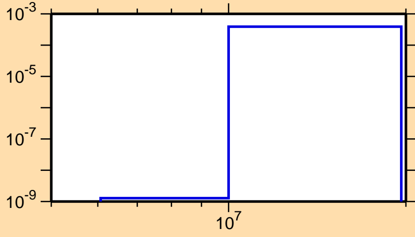
\sigma vs. E for ^{123}\text{Cd}(n,p)
