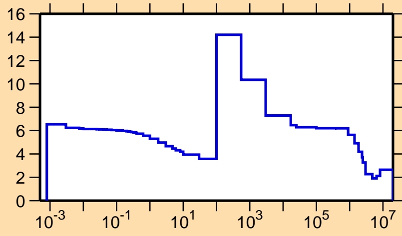
\sigma vs. E for ^{123}\text{Cd}(n,\text{el.})
