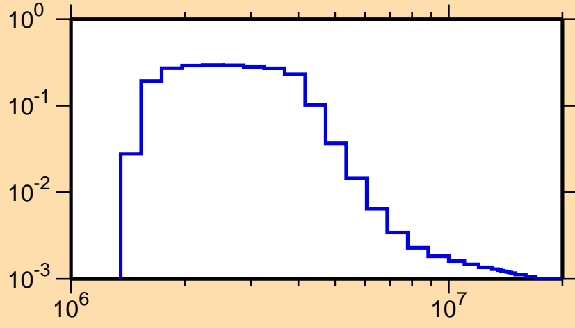
\sigma vs. E for ^{124}\text{Cd}(n,n_3)
