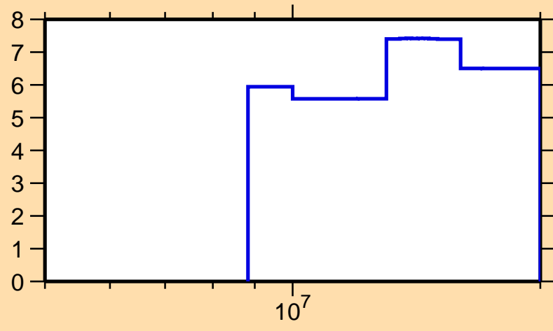
\Delta\sigma/\sigma vs. E for ^{124}\text{Cd}(n,\text{nonel.})
