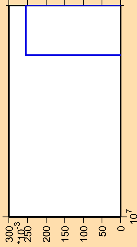
\Delta\sigma/\sigma vs. E for ^{124}\text{Cd}(n,nt)
