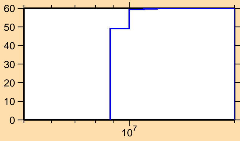
\Delta\sigma/\sigma vs. E for ^{124}\text{Cd}(n,n\text{cont.})
