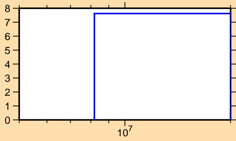
\Delta\sigma/\sigma vs. E for ^{124}\text{Cd}(n,\text{el.})
