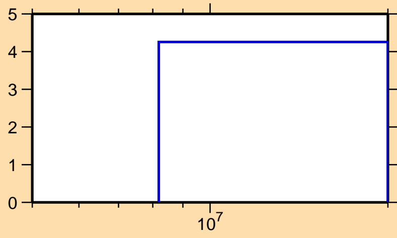
\Delta\sigma/\sigma vs. E for ^{124}\text{Cd}(n,\text{tot.})
