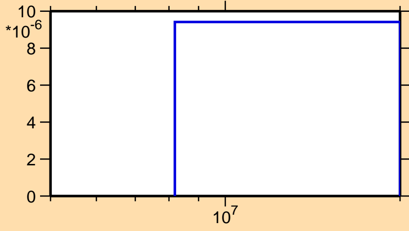
\sigma vs. E for ^{124}\text{Cd}(n,p)
