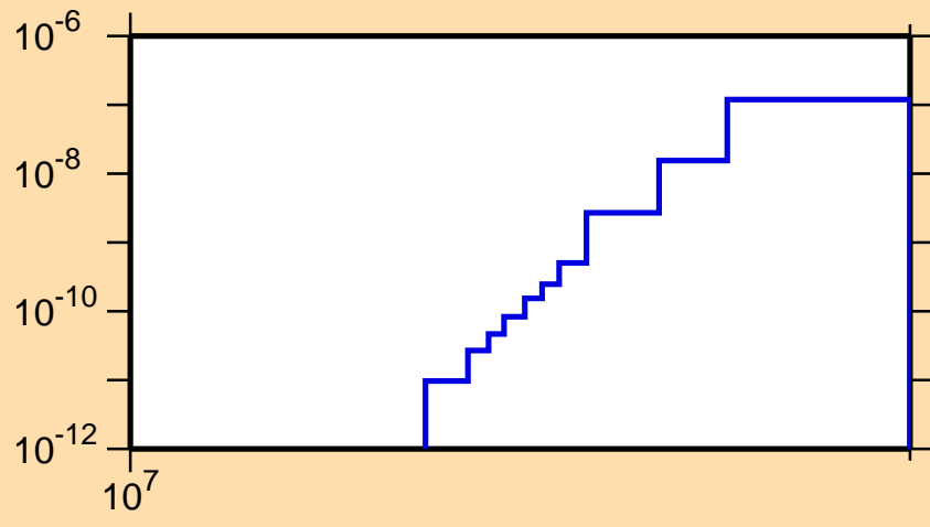
\sigma vs. E for ^{121}\text{Ce}(\text{mt } 34)
