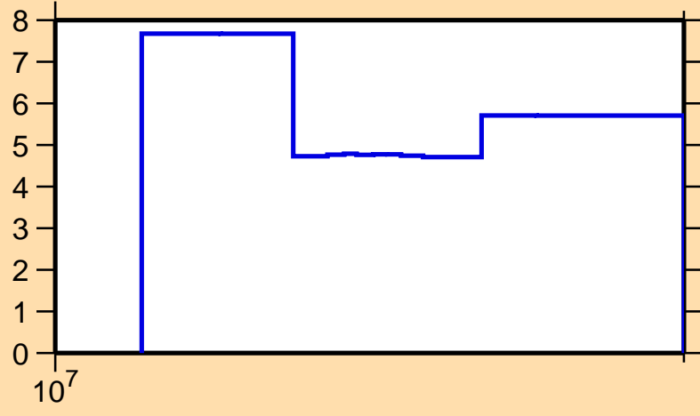
\Delta\sigma/\sigma vs. E for ^{121}\text{Ce}(n,\text{el.})
