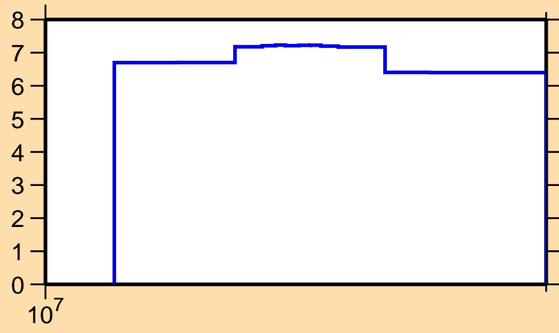
\Delta\sigma/\sigma vs. E for ^{121}\text{Ce}(n,\text{nonel.})
