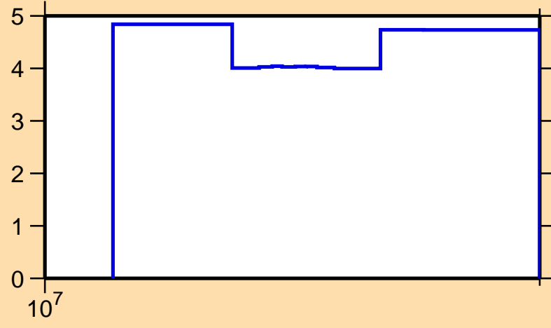
\Delta\sigma/\sigma vs. E for ^{121}\text{Ce}(n,\text{tot.})
