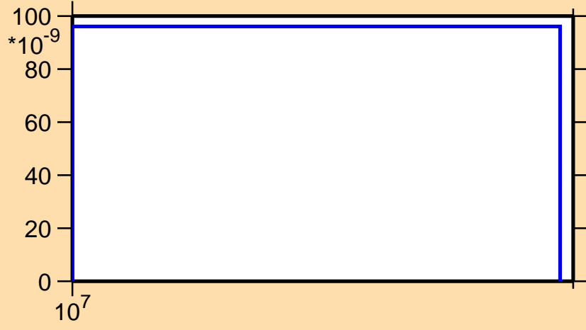
\sigma vs. E for ^{121}\text{Ce}(n,2np)
