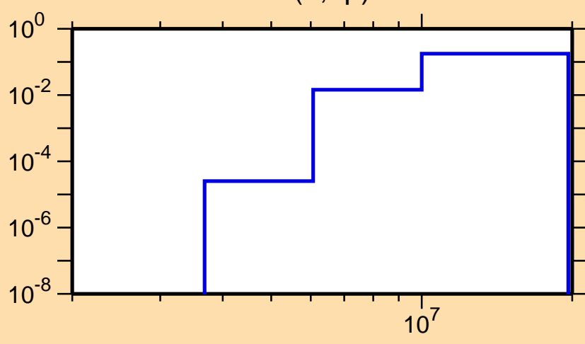
\sigma vs. E for ^{121}\text{Ce}(n,np)
