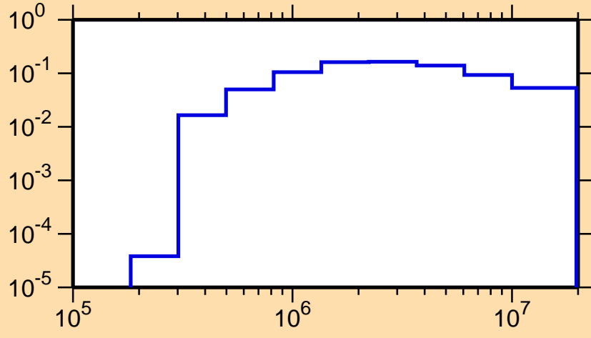
\sigma vs. E for ^{121}\text{Ce}(n,n_1)
