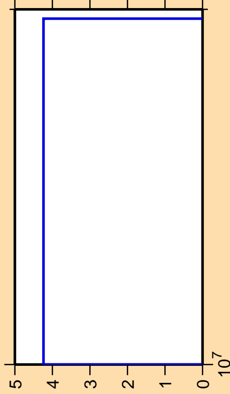
\Delta\sigma/\sigma vs. E for ^{121}\text{Ce}(n,2n\alpha)
