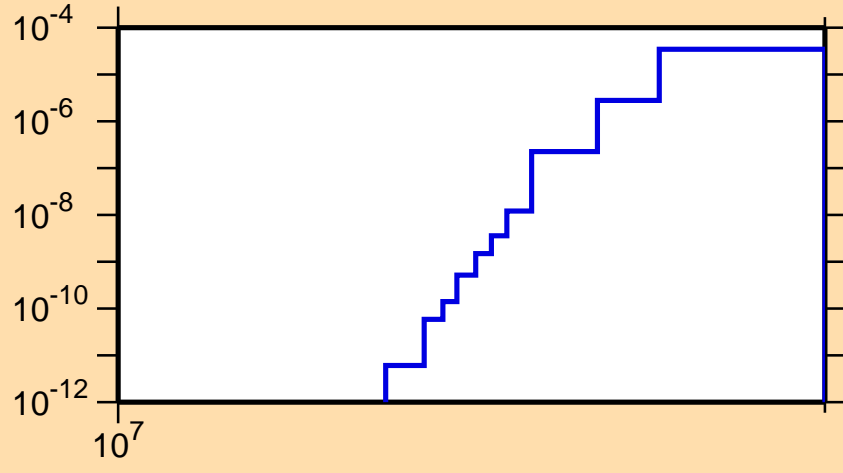
\sigma vs. E for ^{122}\text{Ce}(n,\text{pt})
