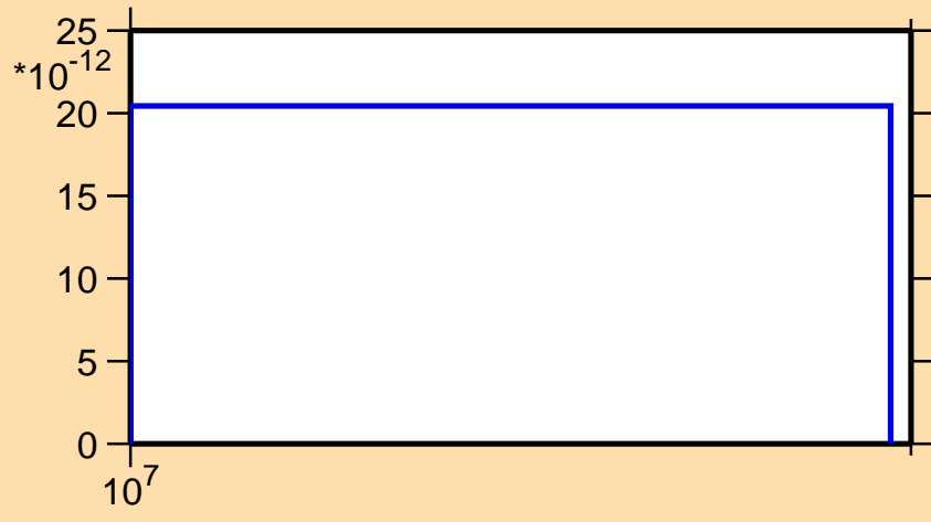
\sigma vs. E for ^{122}\text{Ce} (mt 34)
