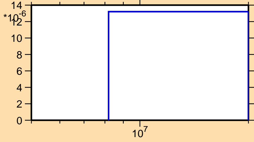
\sigma vs. E for ^{122}\text{Ce}(n,2n)
