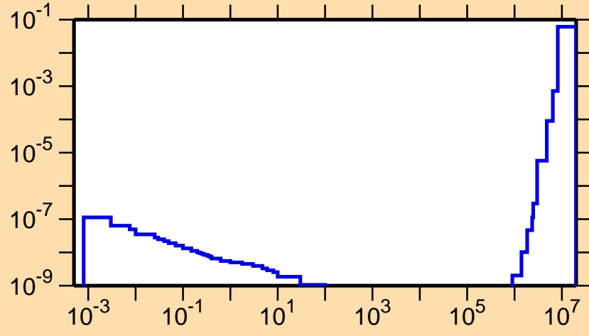
\sigma vs. E for ^{122}\text{Ce}(n, p\alpha)
