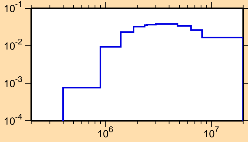
\sigma vs. E for ^{122}\text{Ce}(n,n_2)
