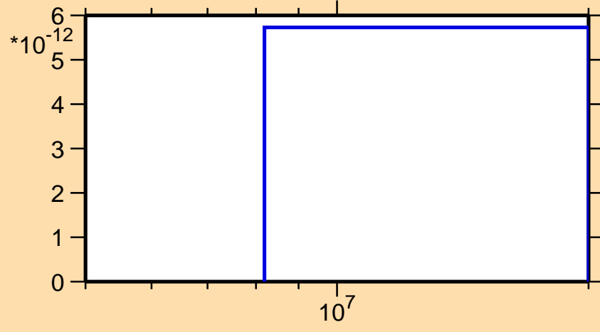
\sigma vs. E for ^{122}\text{Ce}(n,nd)
