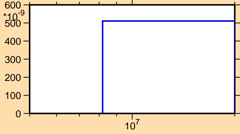
\sigma vs. E for ^{122}\text{Ce}(\text{mt } 45)
