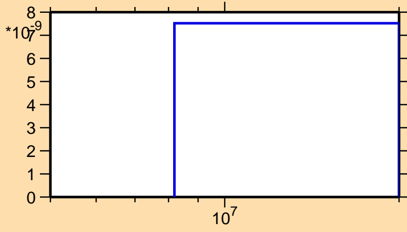
\sigma vs. E for ^{122}\text{Ce}(\text{mt117})
