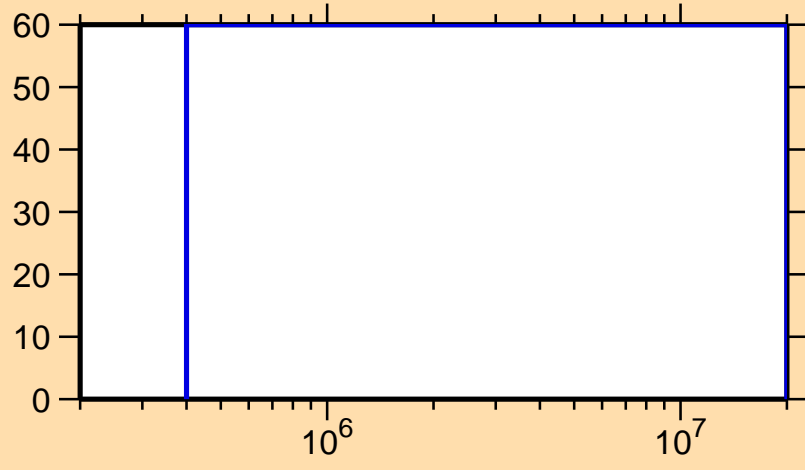
\Delta\sigma/\sigma vs. E for ^{122}\text{Ce}(n,n\text{cont.})
