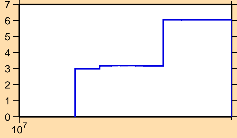
\Delta\sigma/\sigma vs. E for ^{124}\text{Ce}(n,\text{tot.})
