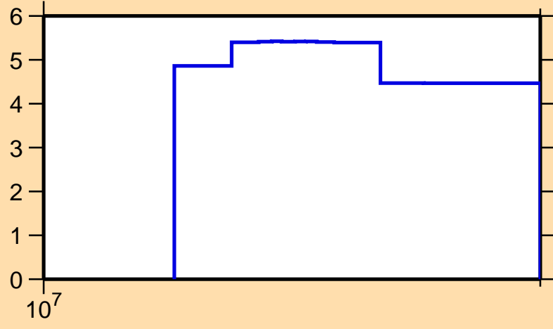
\Delta\sigma/\sigma vs. E for ^{124}\text{Ce}(n,\text{nonel.})
