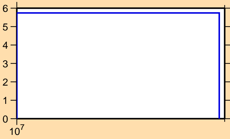
\Delta\sigma/\sigma vs. E for ^{124}\text{Ce}(n,\text{el.})
