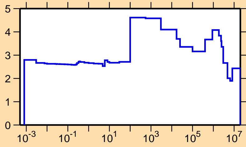
\sigma vs. E for ^{124}\text{Ce}(n,\text{el.})
