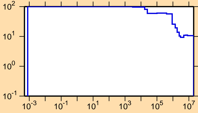
\Delta\sigma/\sigma vs. E for ^{126}\text{Ce}(n,\text{nonel.})
