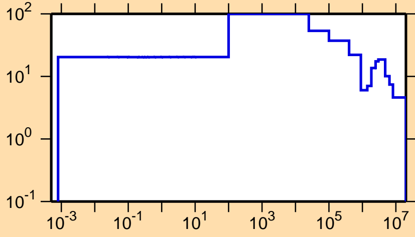
\Delta\sigma/\sigma vs. E for ^{126}\text{Ce}(n,\text{el.})
