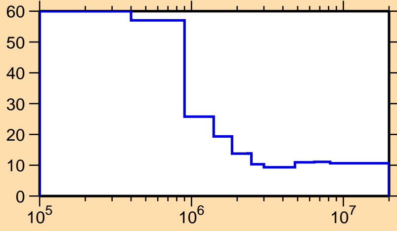
\Delta\sigma/\sigma vs. E for ^{126}\text{Ce}(n,\text{nonel.})
