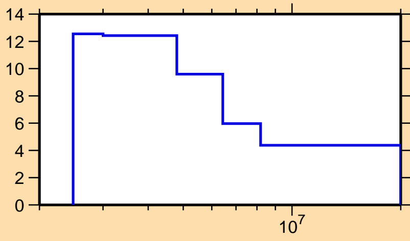
\Delta\sigma/\sigma vs. E for ^{126}\text{Ce}(n,\text{tot.})
