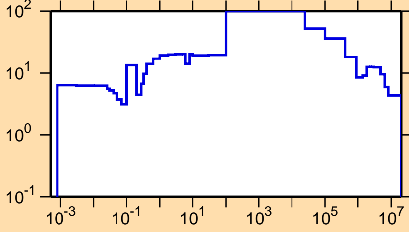
\Delta\sigma/\sigma vs. E for ^{126}\text{Ce}(n,\text{tot.})
