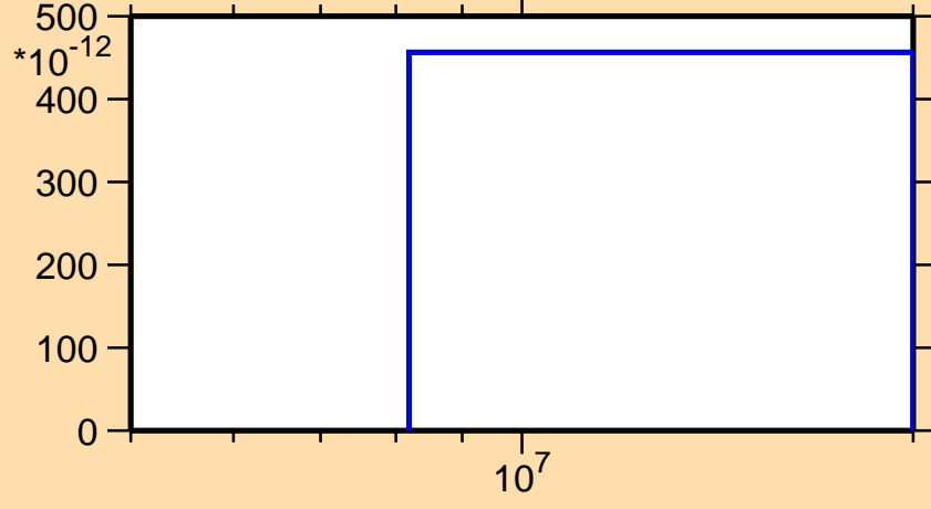
\sigma vs. E for ^{126}\text{Ce}(n,2np)
