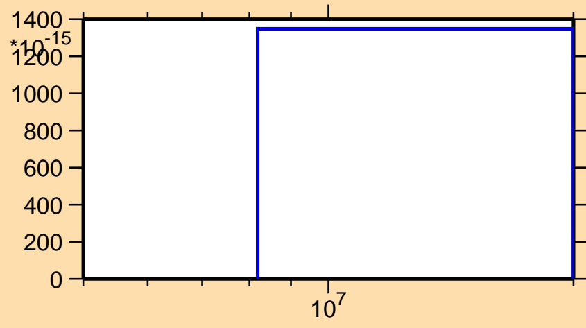
\sigma vs. E for ^{126}\text{Ce} (mt 34)
