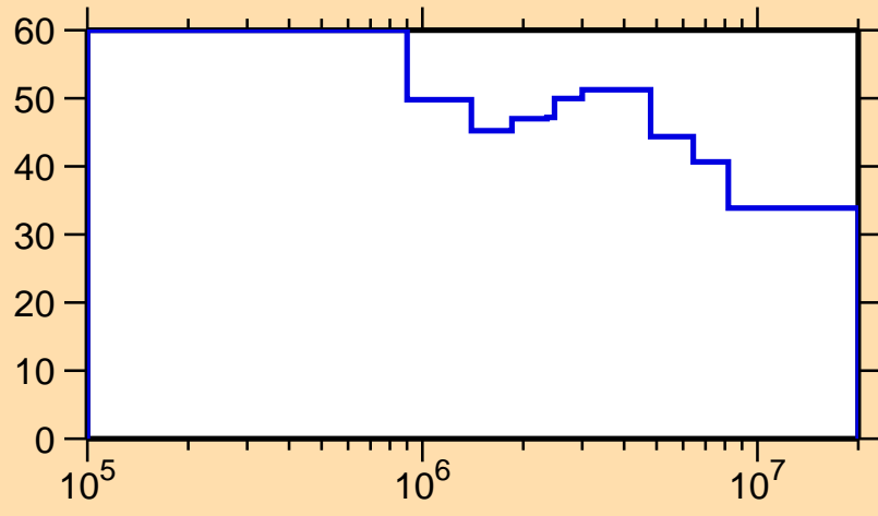
\Delta\sigma/\sigma vs. E for ^{126}\text{Ce}(n,n_1)
