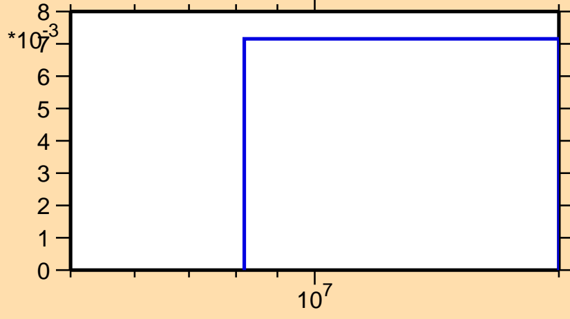
\sigma vs. E for ^{126}\text{Ce}(n,2n)
