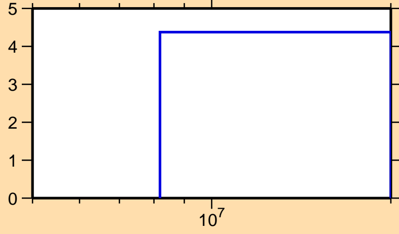
\Delta\sigma/\sigma vs. E for ^{126}\text{Ce}(n,\text{tot.})
