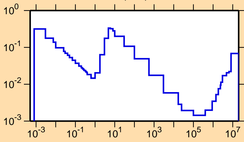
\sigma vs. E for ^{126}\text{Ce}(n,\alpha)
