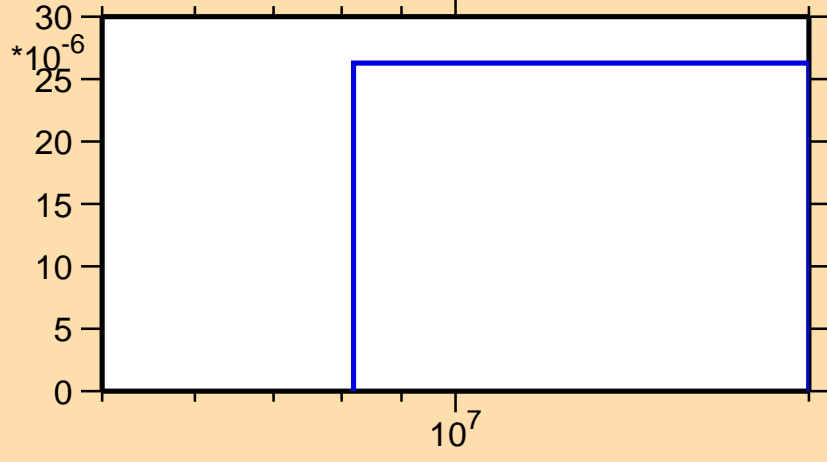
\sigma vs. E for ^{126}\text{Ce}(n,\text{pd})
