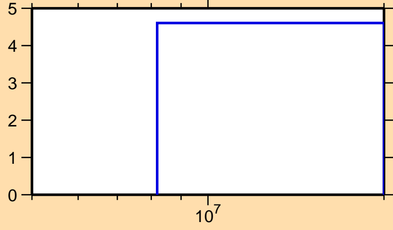
\Delta\sigma/\sigma vs. E for ^{126}\text{Ce}(n,\text{el.})
