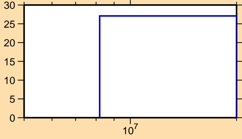
\Delta\sigma/\sigma vs. E for ^{126}\text{Ce}(n,\text{inel.})
