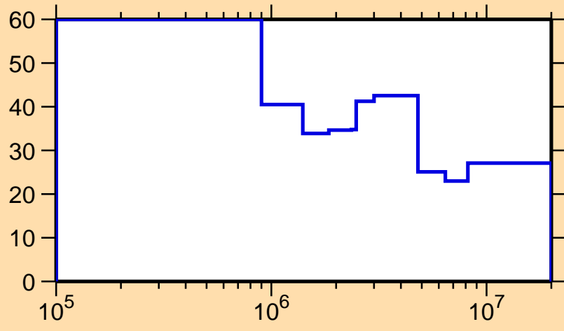
\Delta\sigma/\sigma vs. E for ^{126}\text{Ce}(n,\text{inel.})
