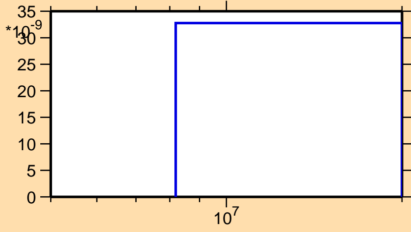
\sigma vs. E for ^{126}\text{Ce}(\text{mt } 45)
