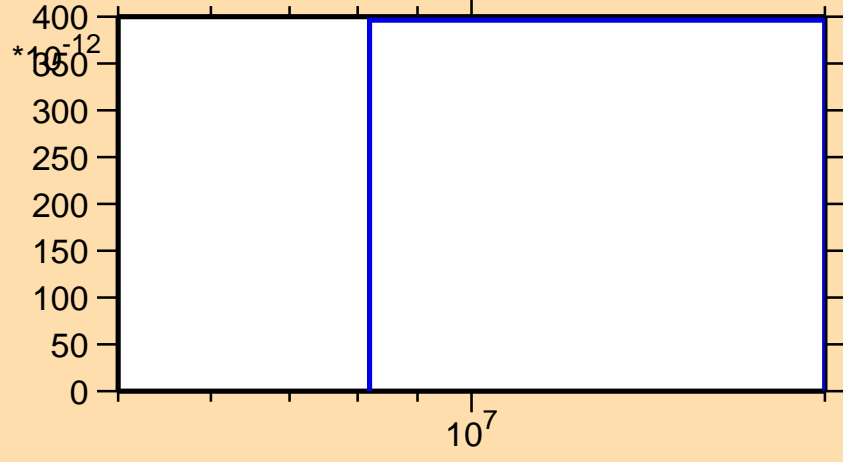
\sigma vs. E for ^{126}\text{Ce}(\text{mt117})
