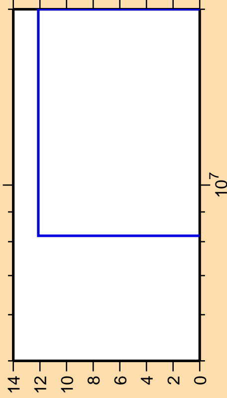
\Delta\sigma/\sigma vs. E for ^{126}\text{Ce} (mt 34)
