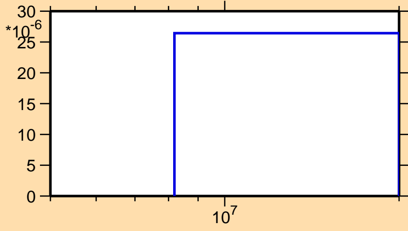
\sigma vs. E for ^{126}\text{Ce}(n,t)
