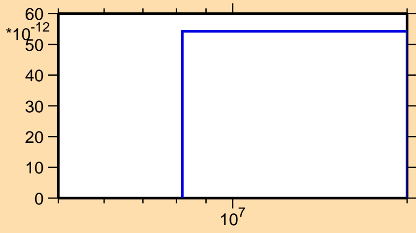
\sigma vs. E for ^{126}\text{Ce}(n,\text{nd})
