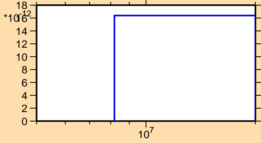
\sigma vs. E for ^{126}\text{Ce}(n,2n\alpha)
