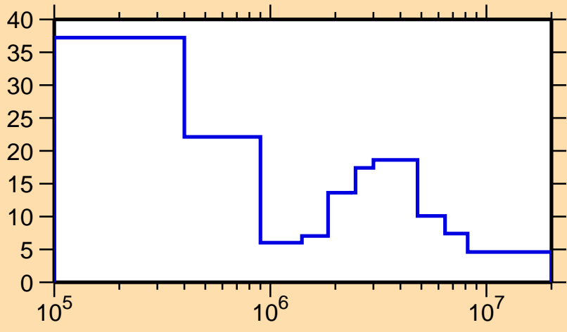
\Delta\sigma/\sigma vs. E for ^{126}\text{Ce}(n,\text{el.})
