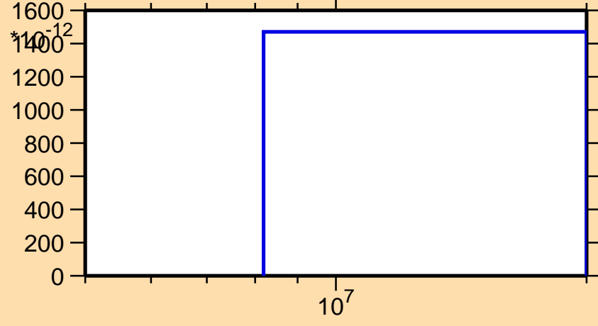
\sigma vs. E for ^{126}\text{Ce}(n,\text{pt})
