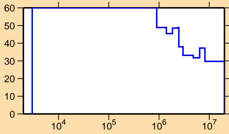
\Delta\sigma/\sigma vs. E for ^{127}\text{Ce}(n,n_1)
