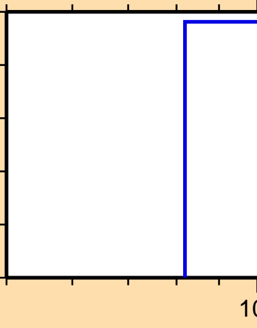
\sigma vs. E for ^{127}\text{Ce}(n,\text{pd})
