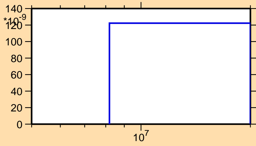
\sigma vs. E for ^{127}\text{Ce}(n,nd)
