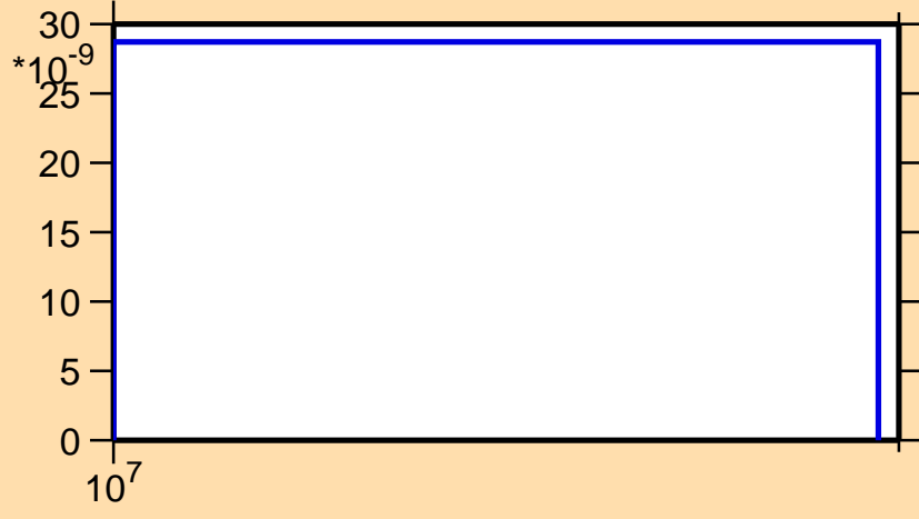
\sigma vs. E for ^{127}\text{Ce} (mt 45)
