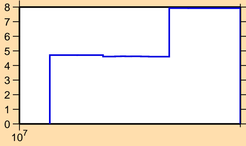
\Delta\sigma/\sigma vs. E for ^{128}\text{Ce}(n,\text{el.})
