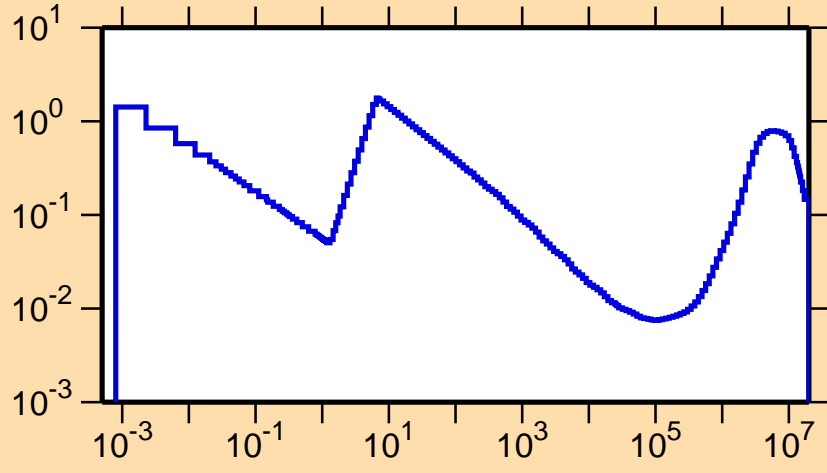
\sigma vs. E for ^{128}\text{Ce}(n,p)
