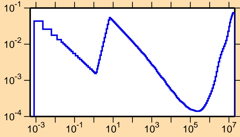
\sigma vs. E for ^{128}\text{Ce}(n,\alpha)
