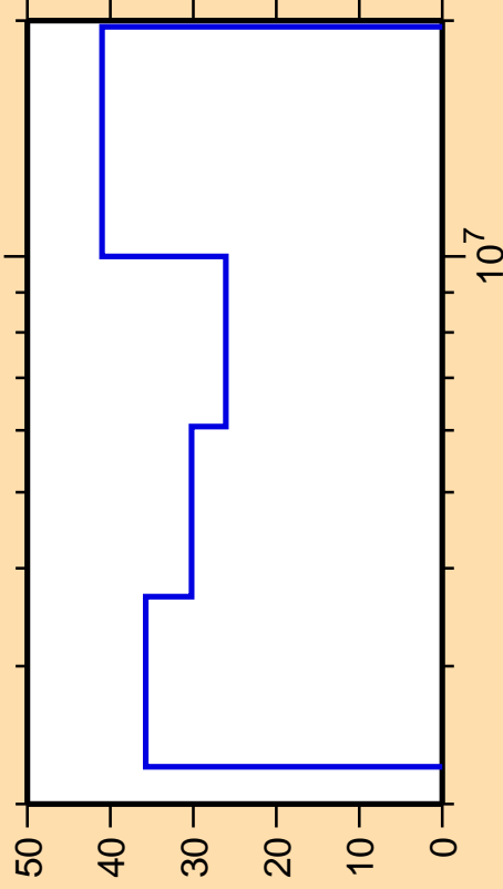
\Delta\sigma/\sigma vs. E for ^{128}\text{Ce}(n,n\text{cont.})
