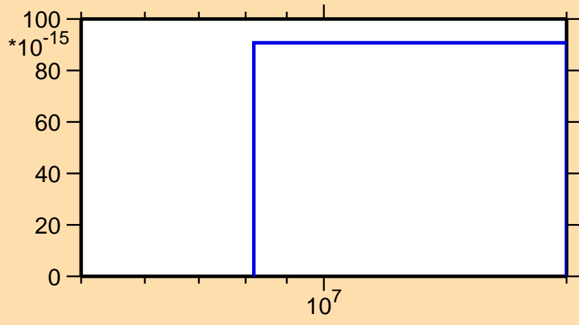
\sigma vs. E for ^{128}\text{Ce}(\text{mt } 34)
