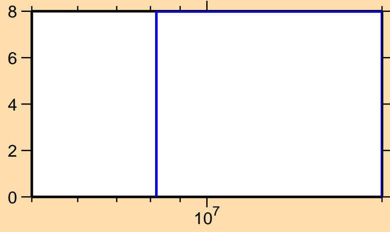
\Delta\sigma/\sigma vs. E for ^{128}\text{Ce}(n,\text{nonel.})
