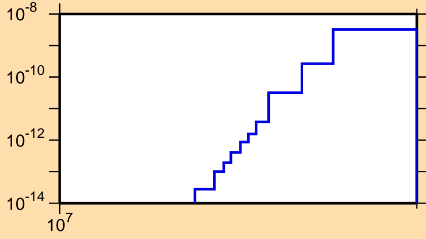
\sigma vs. E for ^{129}\text{Ce}(\text{mt117})
