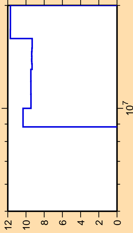
\Delta\sigma/\sigma vs. E for ^{129}\text{Ce}(n,n_1)
