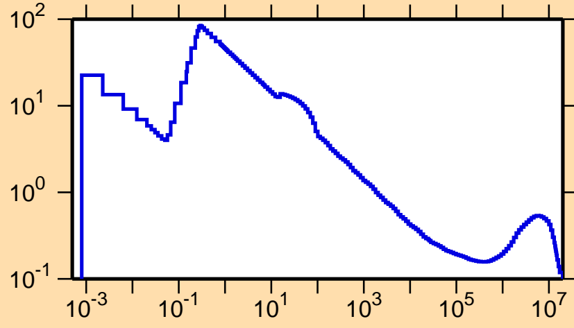
\sigma vs. E for ^{129}\text{Ce}(n,p)
