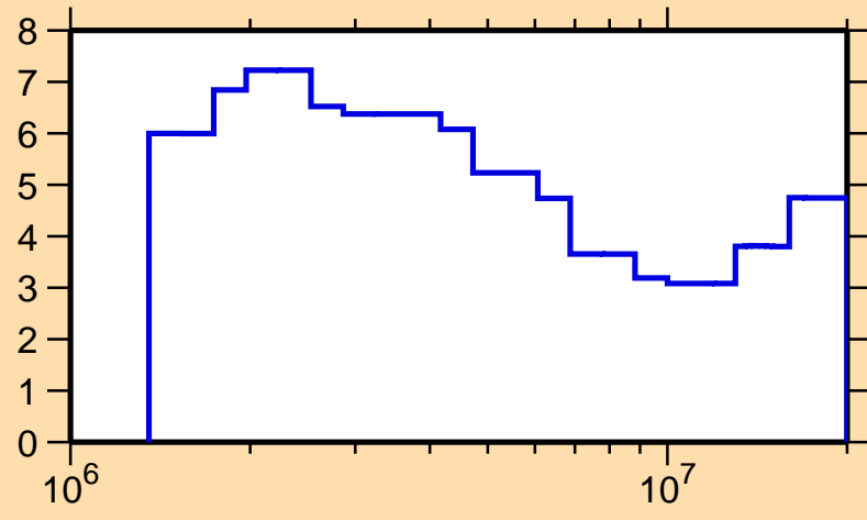
\Delta\sigma/\sigma vs. E for ^{129}\text{Ce}(n,\text{tot.})
