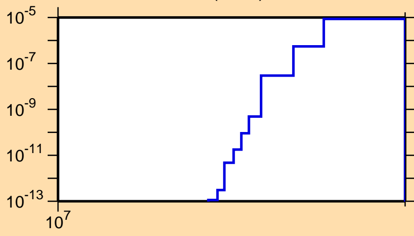
\sigma vs. E for ^{129}\text{Ce}(n,\text{nd})
