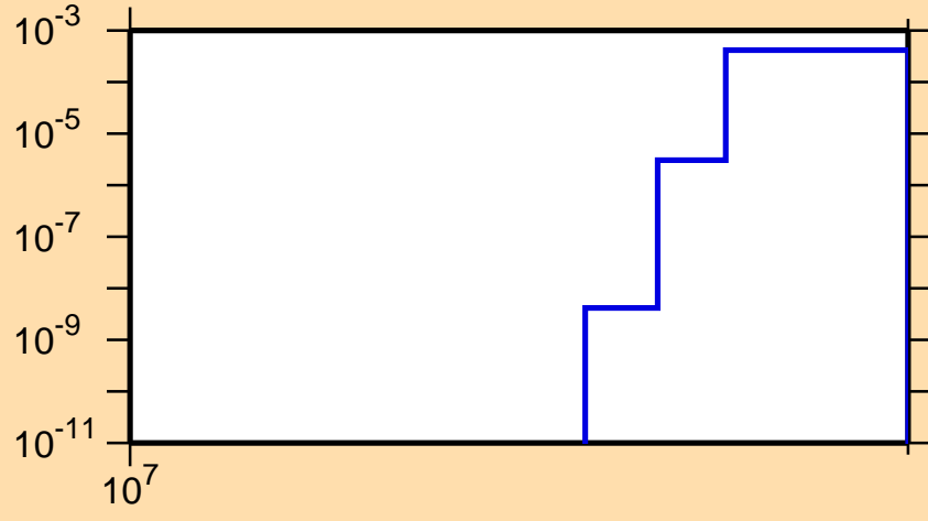
\sigma vs. E for ^{129}\text{Ce}(n,2np)
