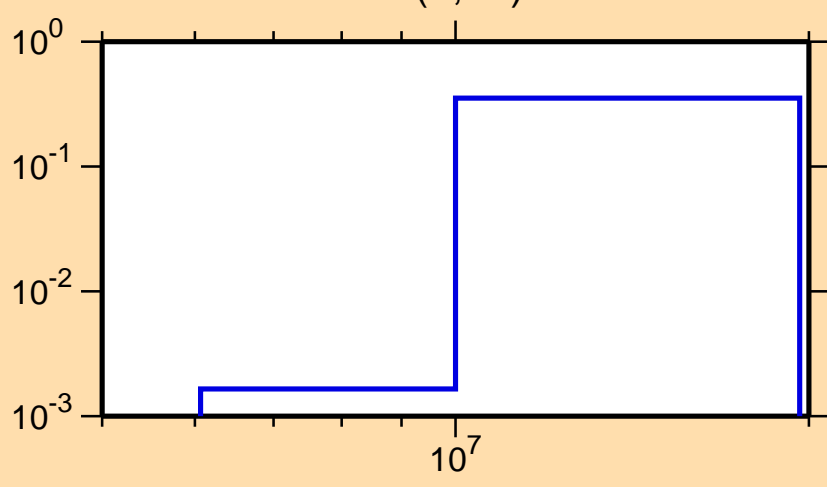
\sigma vs. E for ^{129}\text{Ce}(n,2n)
