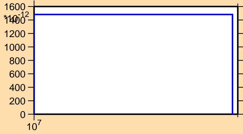
\sigma vs. E for ^{129}\text{Ce} (mt 45)
