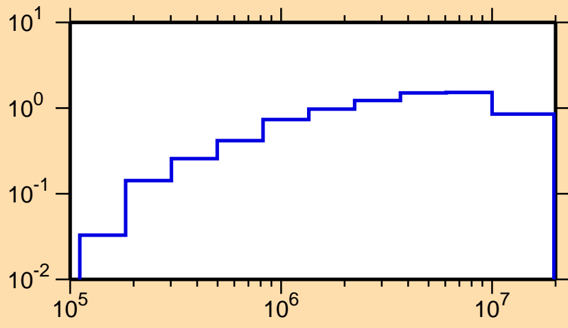
\sigma vs. E for ^{129}\text{Ce}(n,\text{inel.})
