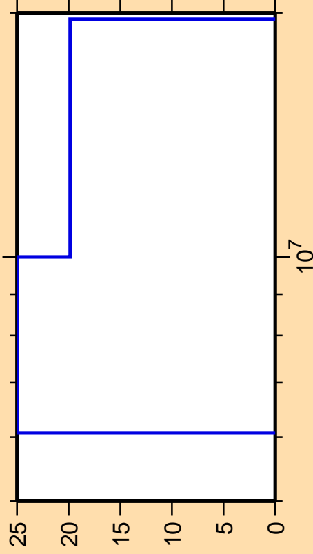
\Delta\sigma/\sigma vs. E for ^{129}\text{Ce}(n,n\text{cont.})
