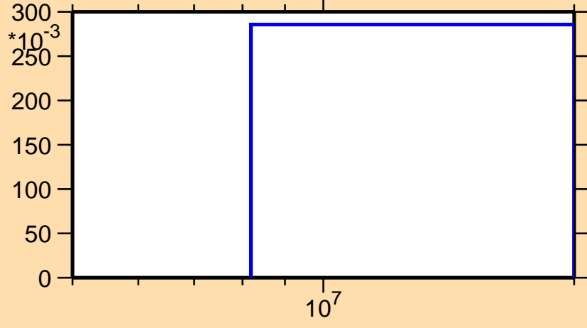
\sigma vs. E for ^{129}\text{Ce}(n,2n)
