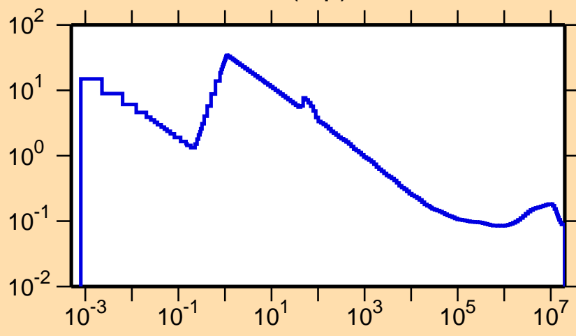
\sigma vs. E for ^{131}\text{Ce}(n,p)
