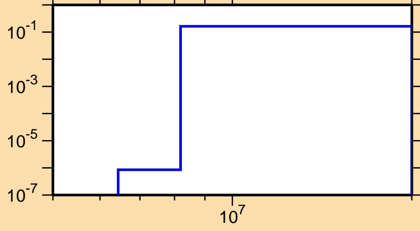
\sigma vs. E for ^{131}\text{Ce}(n,np)
