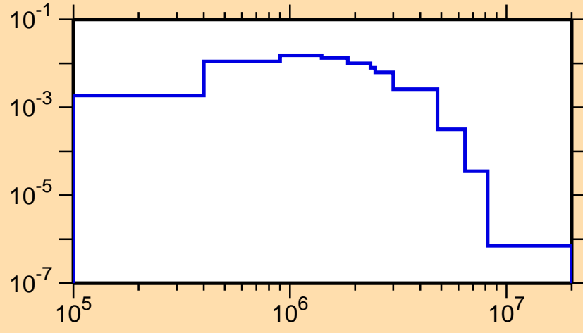
\sigma vs. E for ^{131}\text{Ce}(n,n_3)
