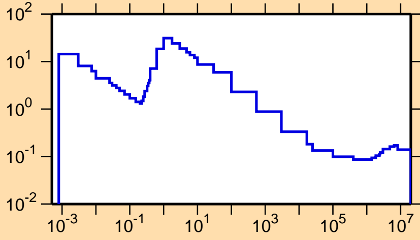
\sigma vs. E for ^{131}\text{Ce}(n,p)
