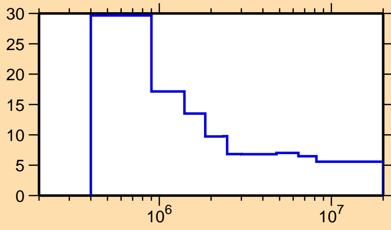
\Delta\sigma/\sigma vs. E for ^{131}\text{Ce}(n,\text{nonel.})
