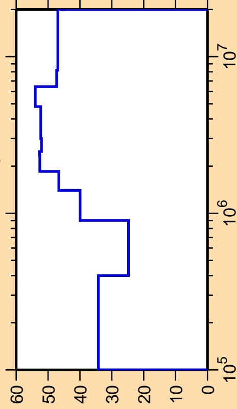
\Delta\sigma/\sigma vs. E for ^{131}\text{Ce}(n,n_3)
