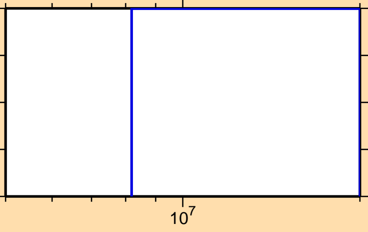
\sigma vs. E for ^{133}\text{Ce}(n,t)
