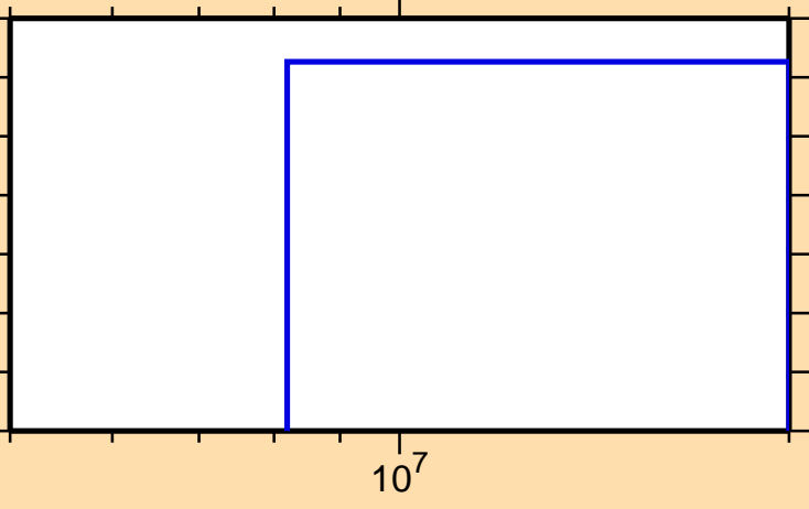
\sigma vs. E for ^{133}\text{Ce}(n,3n)
